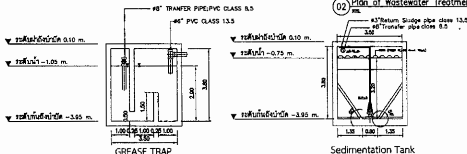
03 Section B-B of Wastewater Treatment Plant
