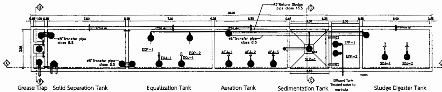
01 Plan of Wastewater Treatment Plant
