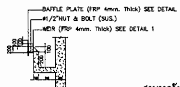
DETAIL OVERFLOW WEIR SCALE NTS
