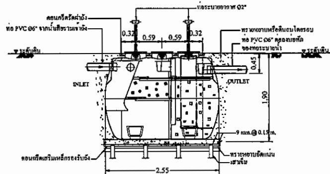
SECTION
