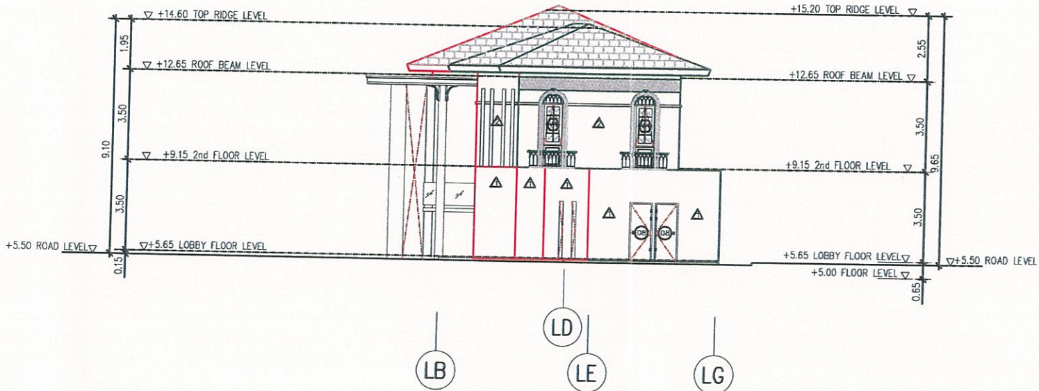
ELEVATION.2 SCALE 1 : 200
