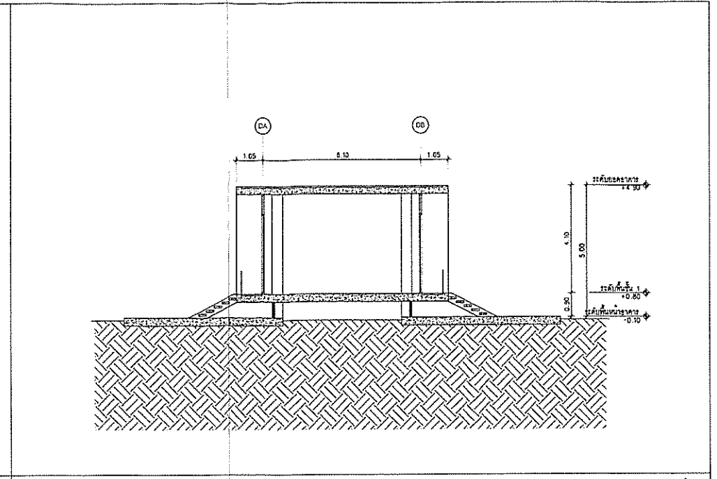
SECTION 4 SCALE 1:100
