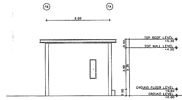
ELEVATION 6 SCALE 1:100
