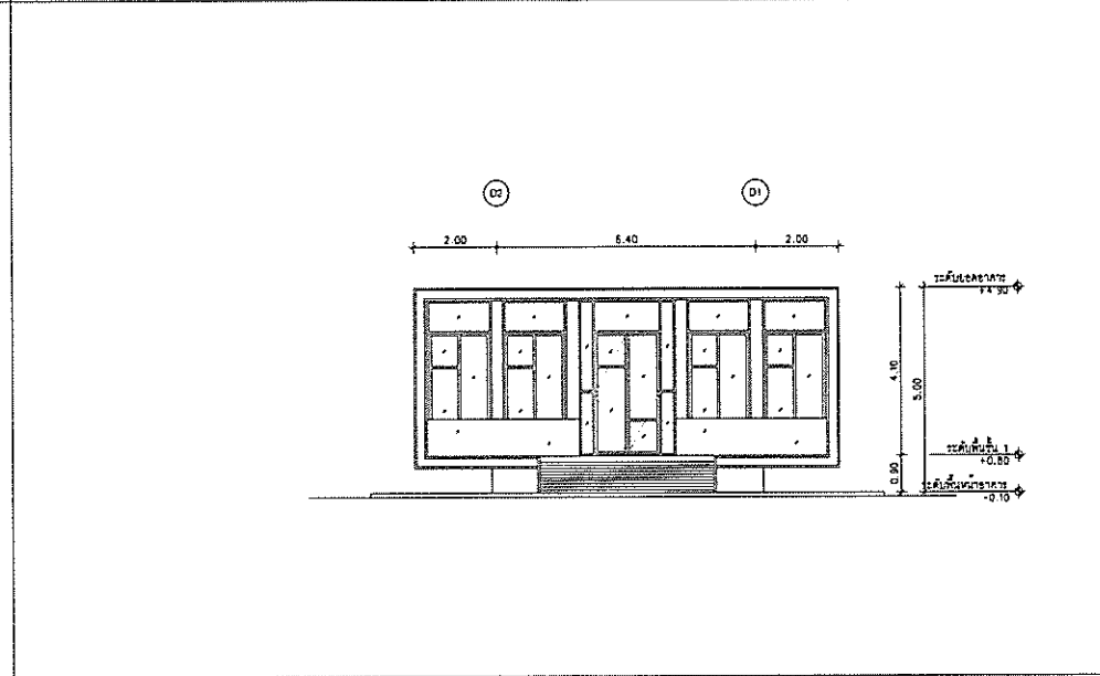
ELEVATION 5 SCALE 1:100
