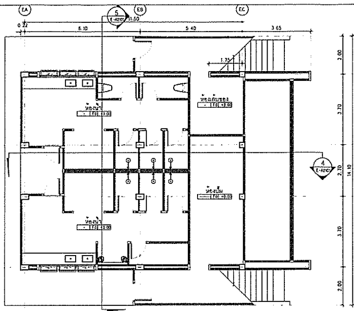
1ST FLOOR PLAN SCALE 1:100
