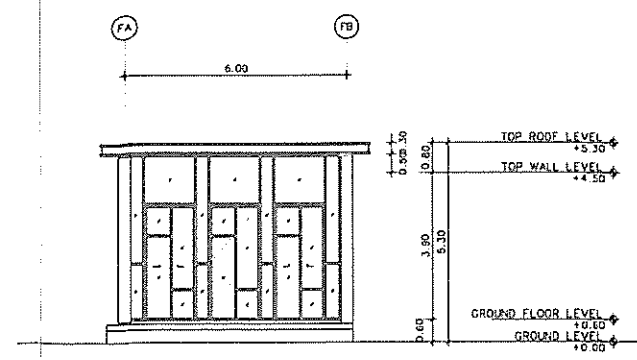
ELEVATION 5 SCALE 1:100
