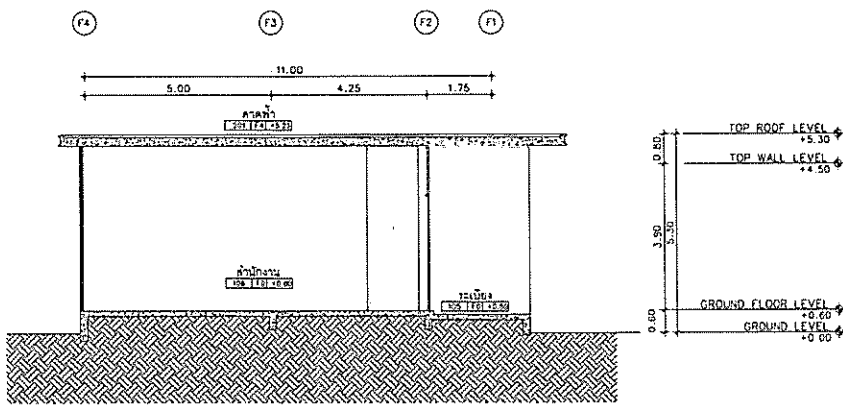
SECTION 4 SCALE 1:100
