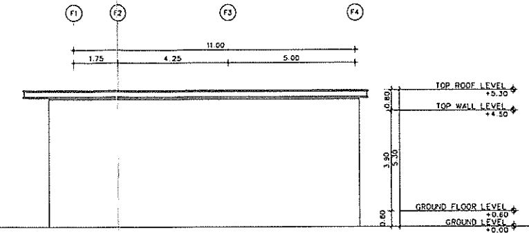
ELEVATION 6 SCALE 1:100
