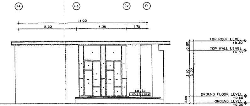
ELEVATION 7 SCALE 1:100
