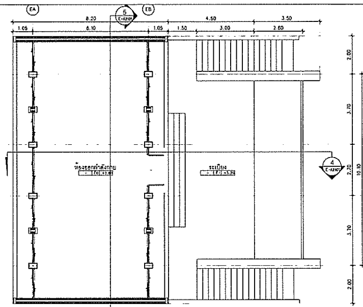
2ND FLOOR PLAN SCALE 1:100
