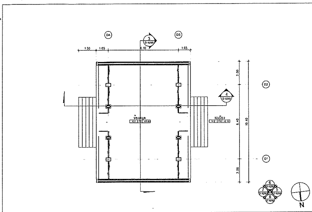
1ST FLOOR PLAN SCALE 1:100
