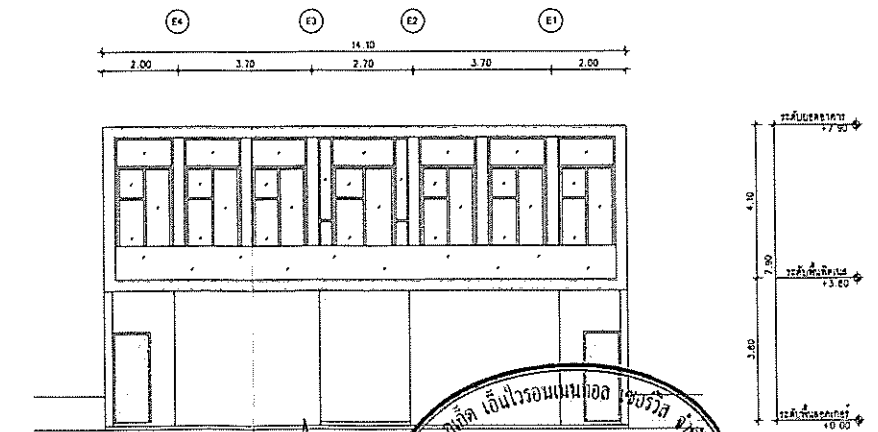
ELEVATION 7 SCALE 1:100
