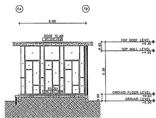
SECTION 3 SCALE 1:100
