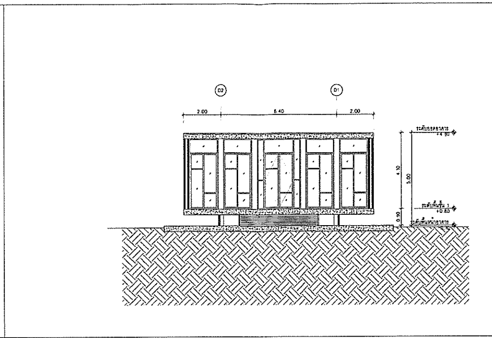
SECTION 3 SCALE 1:100
