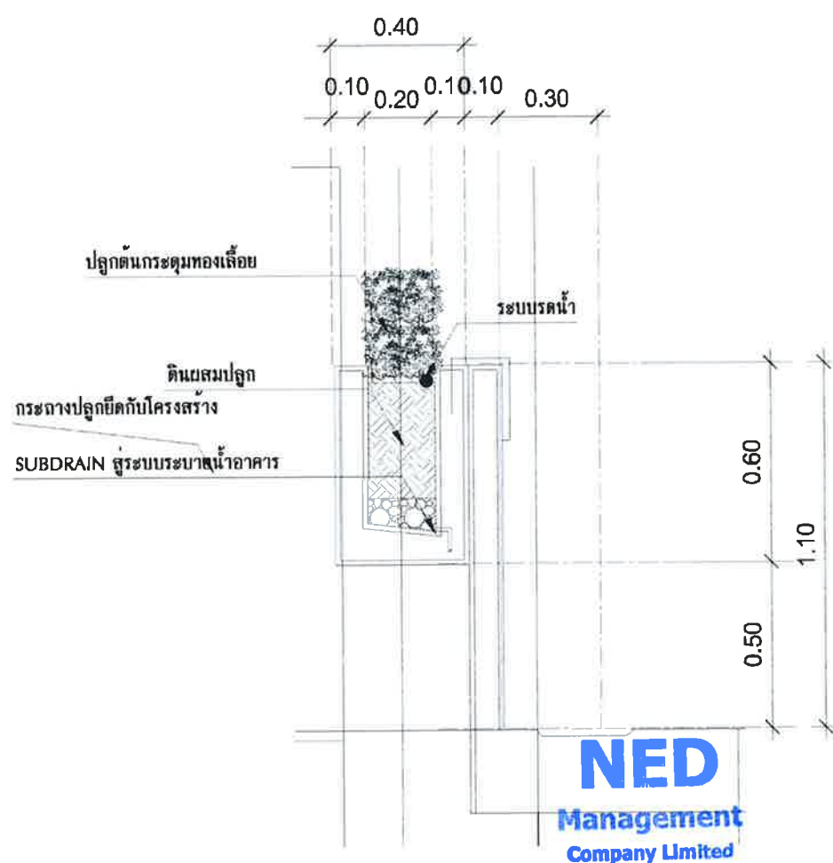
DETAIL SCALE 1:20
